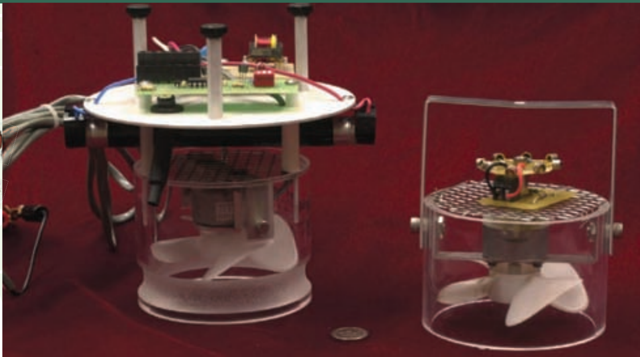
The LED-based insect trap (right) is smaller and lighter and uses less energy than traditional light-based collection devices.
